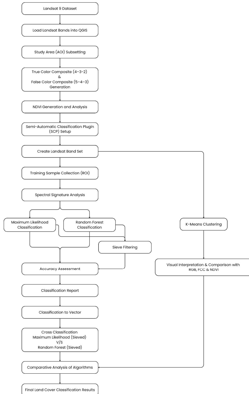
Figure 4.1: QGIS Workflow Diagram
